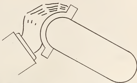
Fig. 5—Method of rocking cap bearing or connecting rod bearing on crank pin by hand.
